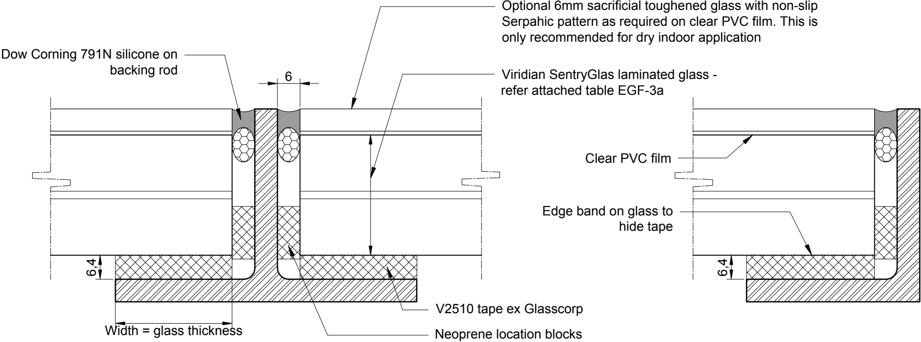
INTERMEDIATE STEEL SUPPORT
